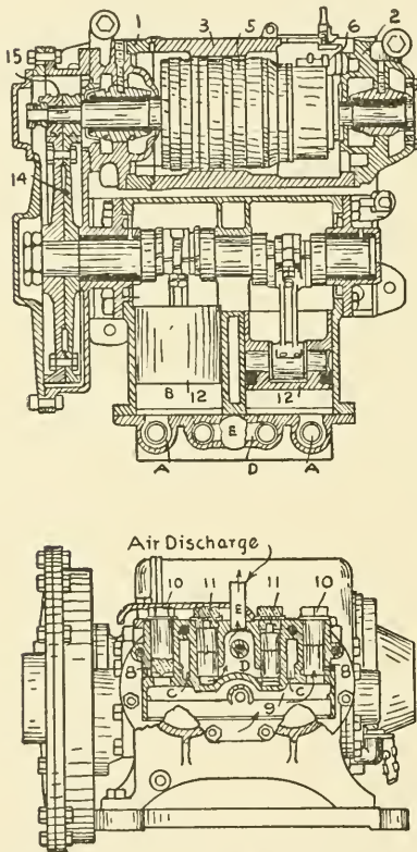
Fig. 87. Section of Motor and Pump in Motor Driven from Pressure
